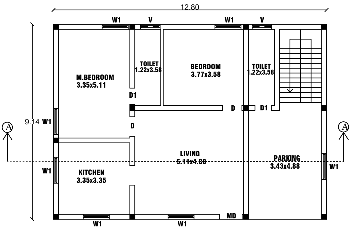
GROUND FLOOR PLAN EAST FACING PLAN
