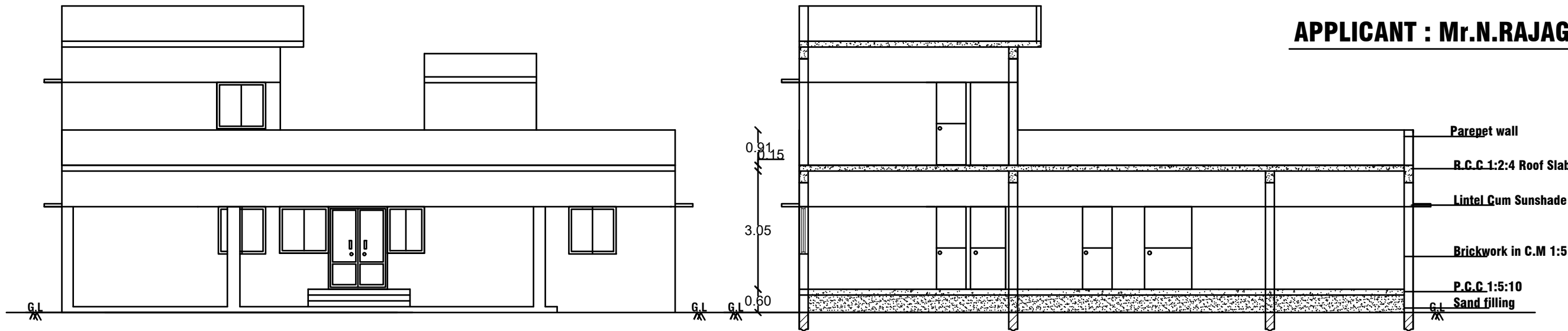
FRONT ELEVATION
