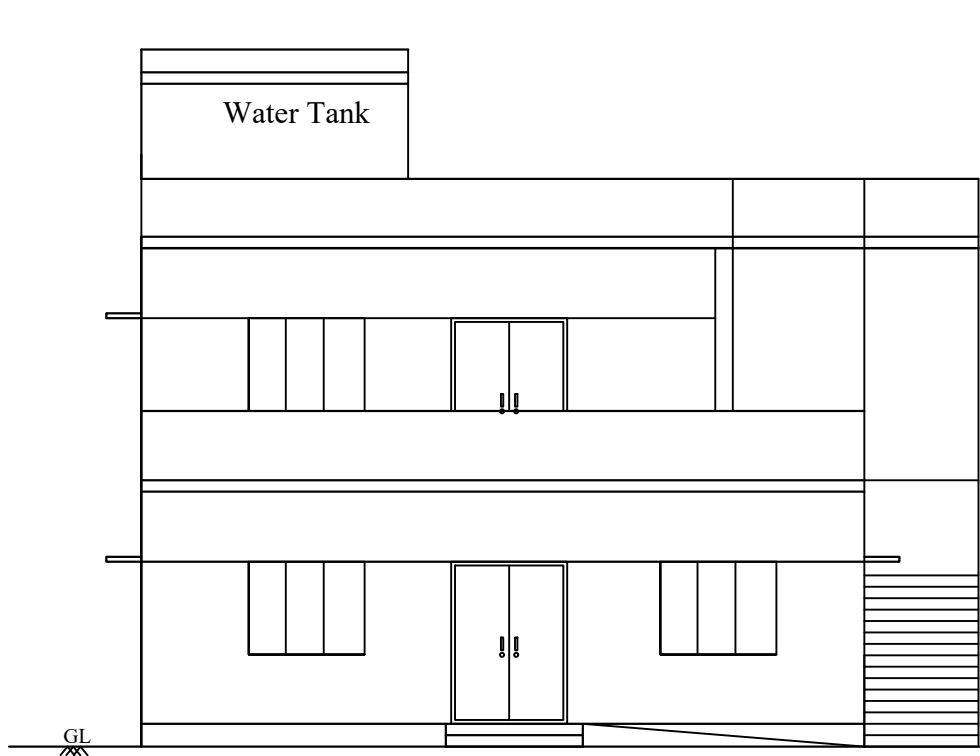
FRONT ELEVATION
