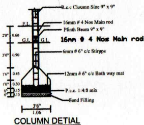
COLUMN DETAIL
