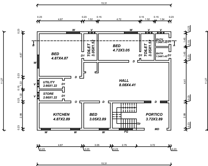
PROPOSED GROUND FLOOR PLAN PLAN ]
