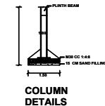
COLUMN DETAILS
