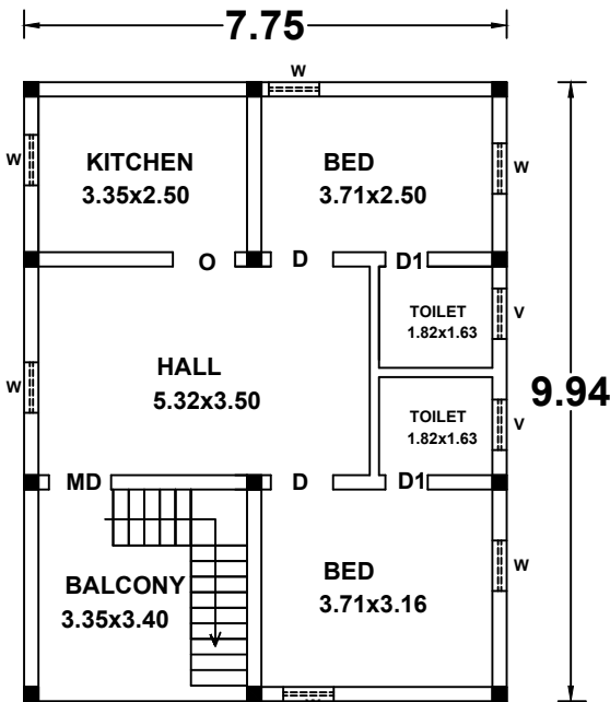
PROPOSED FIRST FLOOR PLAN ( Residential )
