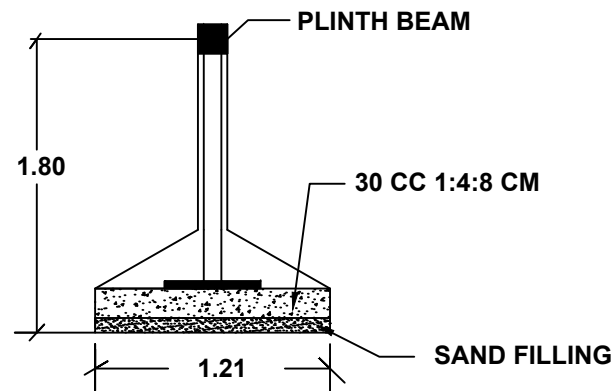
COLUMN DETAILS
