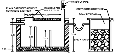
SECTION X-X
