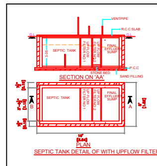
SEPTIC TANK DETAIL OF WITH UPFLOW FILTER
