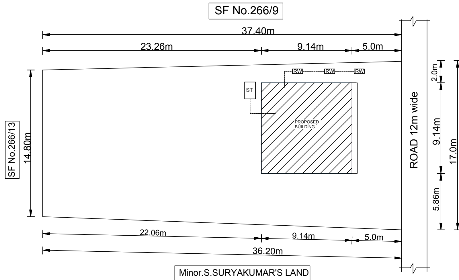
SITE PLAN
