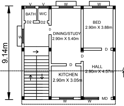
FIRST FLOOR PLAN (Residential Building)
