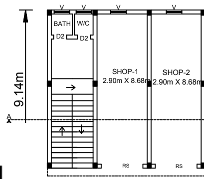
GROUND FLOOR PLAN (Commercial Building)
