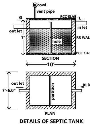
DETAILS OF SEPTIC TANK
