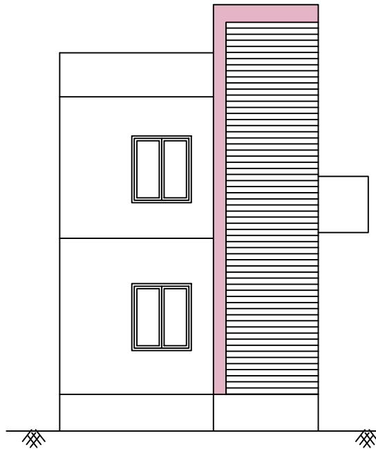
FRONT ELEVATION
