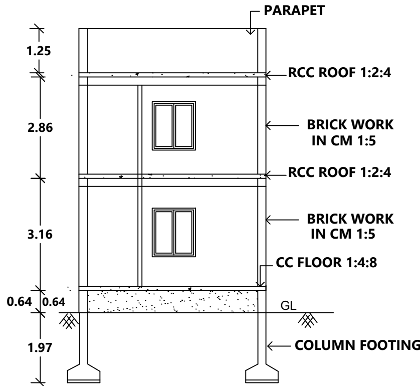
SECTION AB
