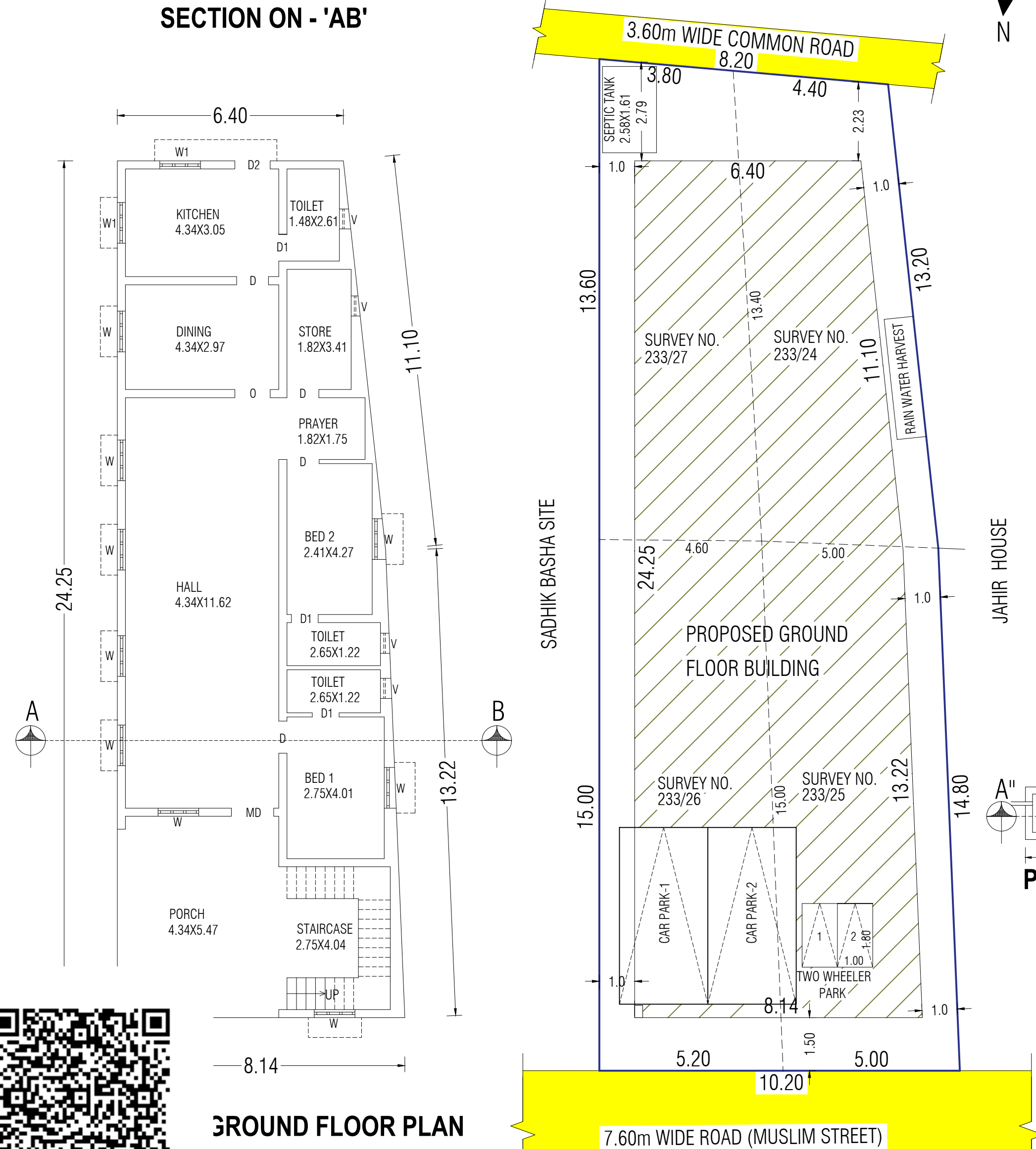
SITE PLAN
