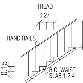
STAIRCASE DETAILS
