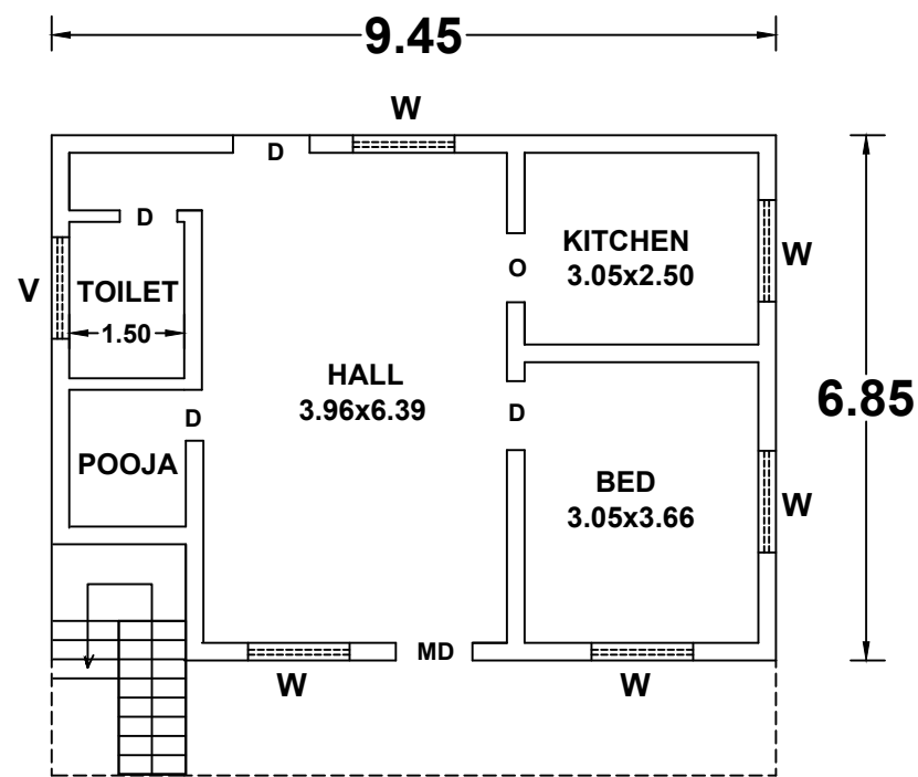
PLAN- GROUND FLOOR
