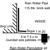
Rain Water Percolation pit
