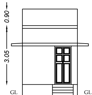
FRONT ELEVATION
