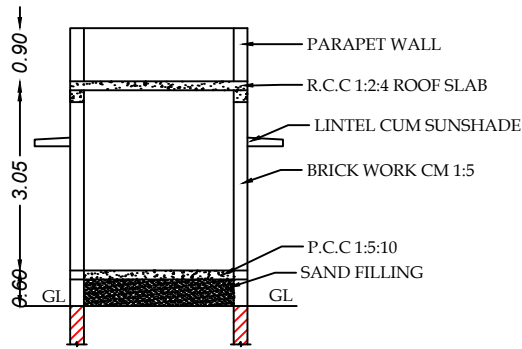
SECTION AB
