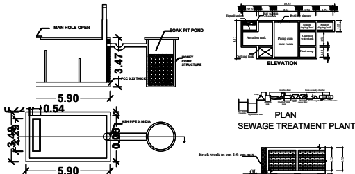
DETAIL OF SEPTIC TANK
