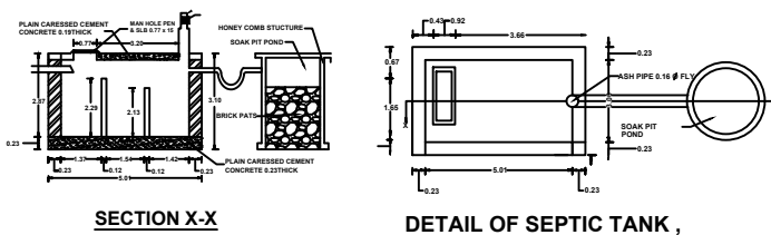
SECTION X-X
