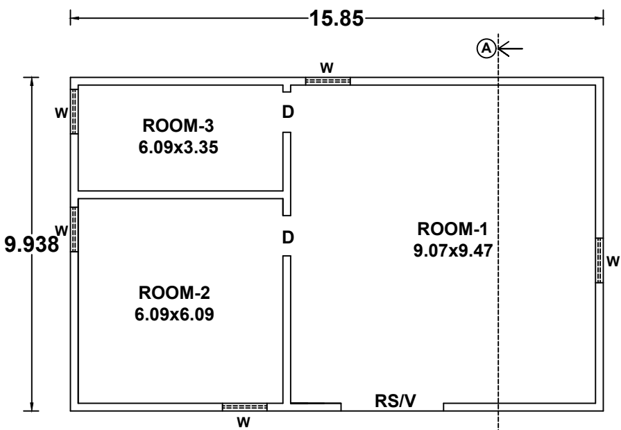
PLAN OF COMMERCIAL BUILDING FACING SOUTH
