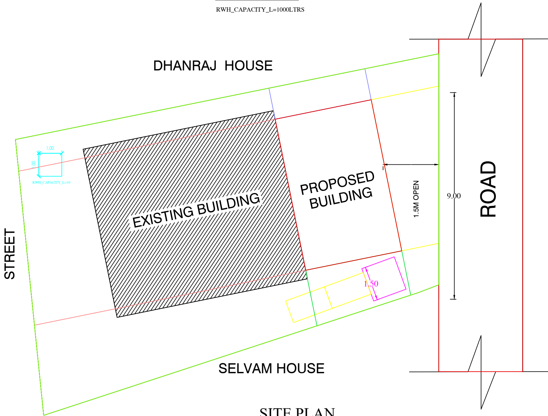
SITE PLAN
