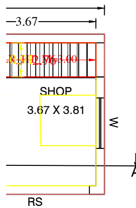
D FLOOR PLAN
