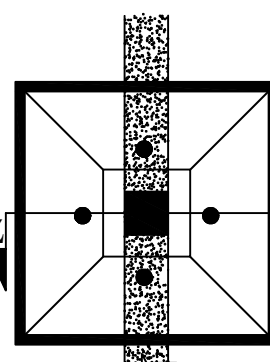
COLUMN FOOTING DETAIL
