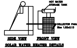
SOLAR WATER HEATER DETAILS
