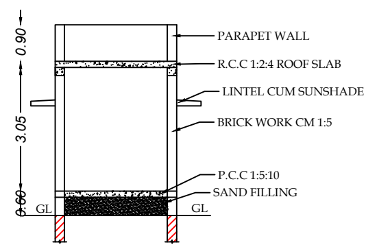
SECTION AB
