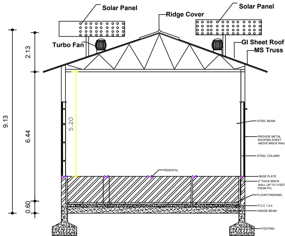
SECTION ON-AA
