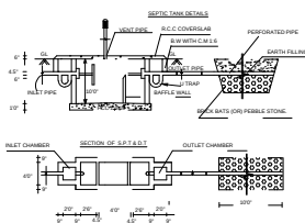
SECTION OF R.C.C 1:2:4
