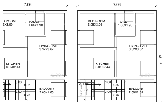
IRST FLOOR
