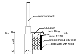
PLINTH BOUNDARY PERCOLATION PIT
