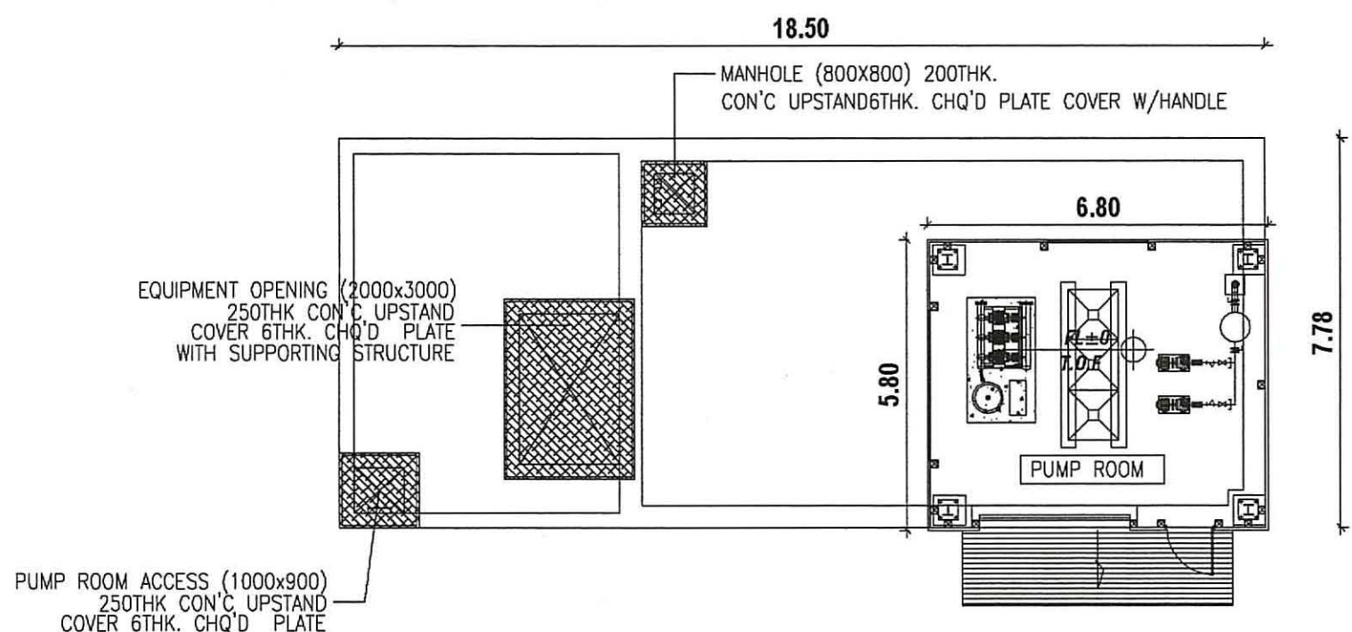
2 GROUND FLOOR PLAN SCALE: 1/100
