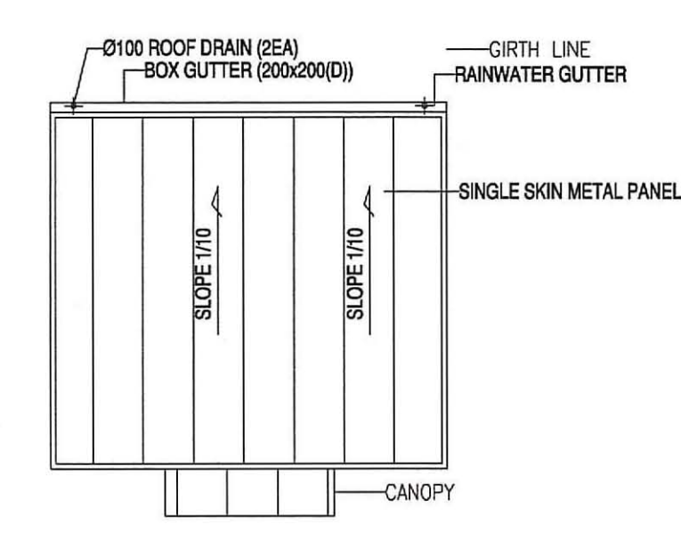
1 ROOF PLAN SCALE: 1/100
