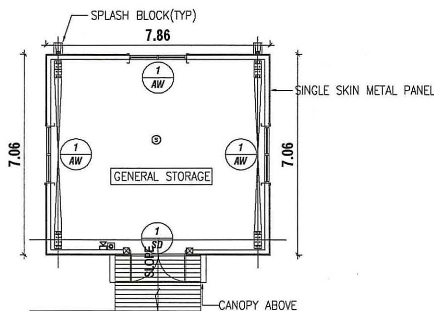
1 GROUND FLOOR PLAN SCALE: 1/100
