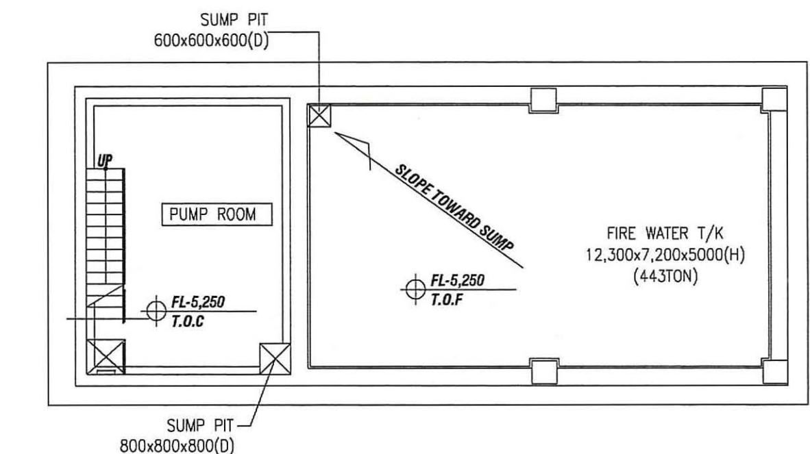
1 BASEMENT LAYOUT SCALE: 1/100
