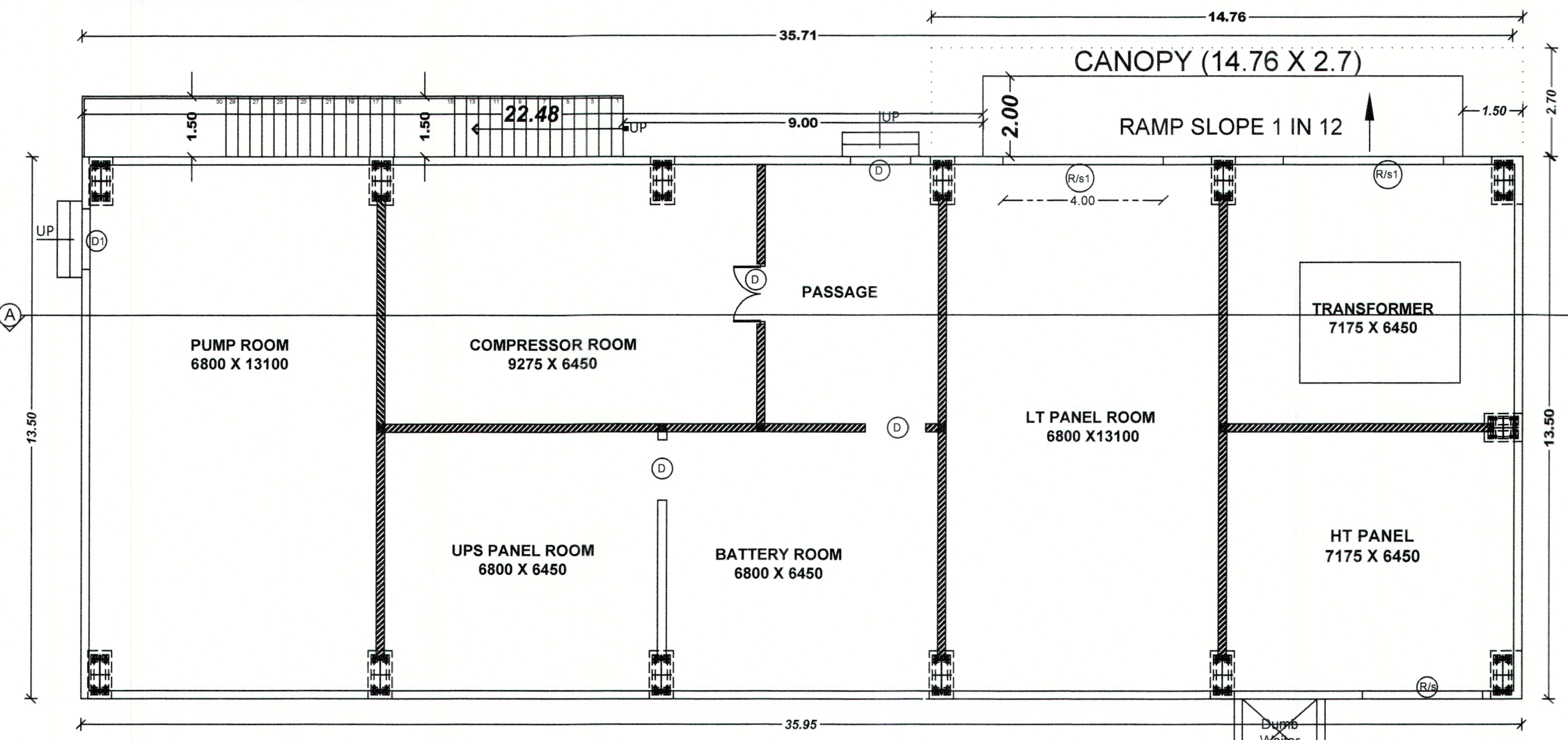
GROUND FLOOR LAYOUT
