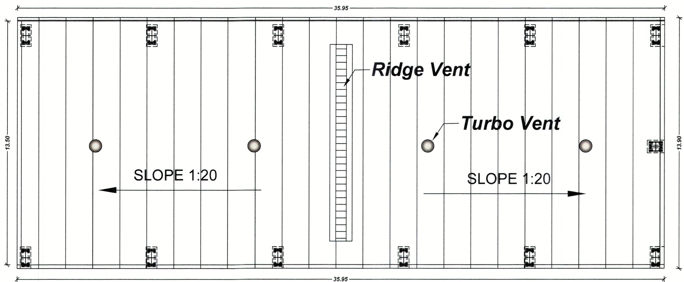
ROOF PLAN
