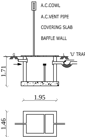
SEPTIC TANK
