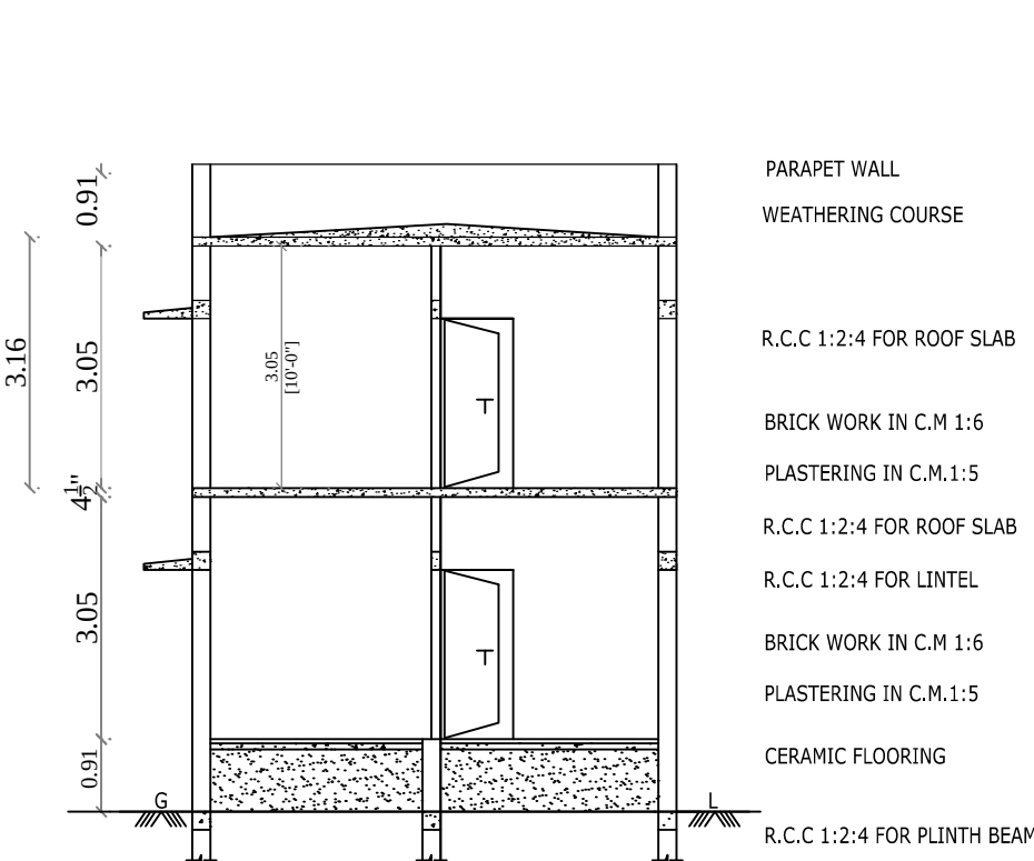
SECTION ON "SC"
