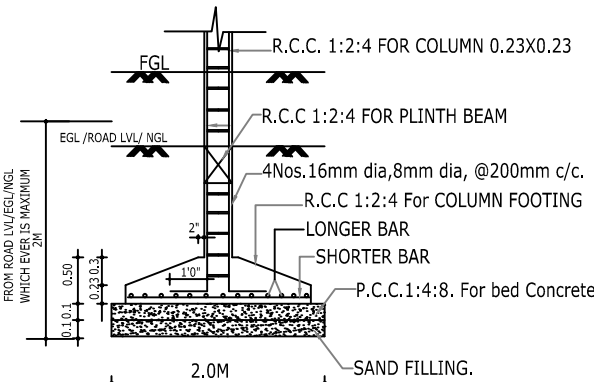
FOUNDATION DETAIL
