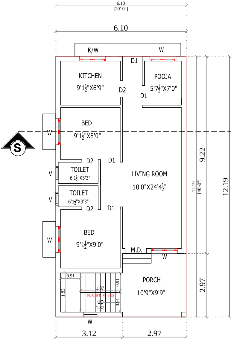
EXTG.,GROUND FLOOR PLAN
