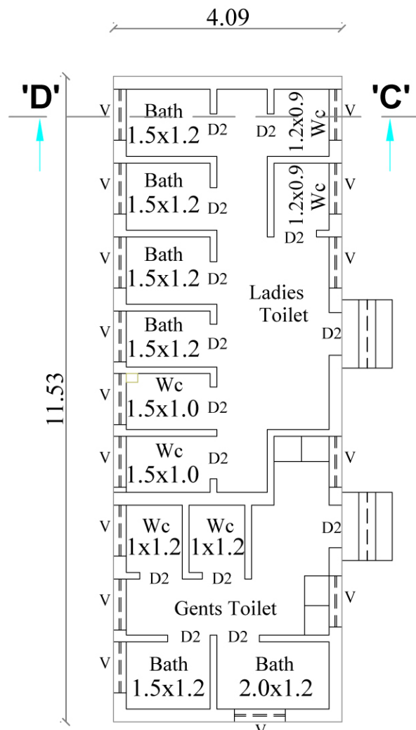
GROUND FLOOR PLAN BLOCK No. 2
