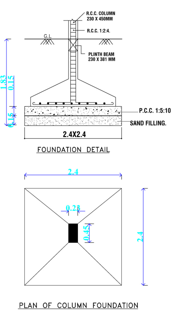
FOUNDATION DETAIL PLAN OF COLUMN FOUNDATION
