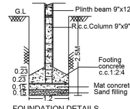
FOUNDATION DETAILS (SCALE: 1" = 4'-0")
