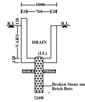
TYPICAL SECTION OF PERCOLATION PIT
