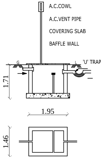
SEPTIC TANK
