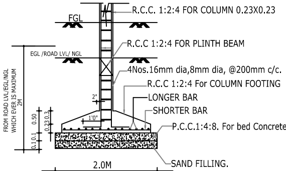
FOUNDATION DETAIL
