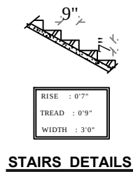
STAIRS DETAILS
