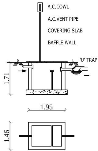
SEPTIC TANK
