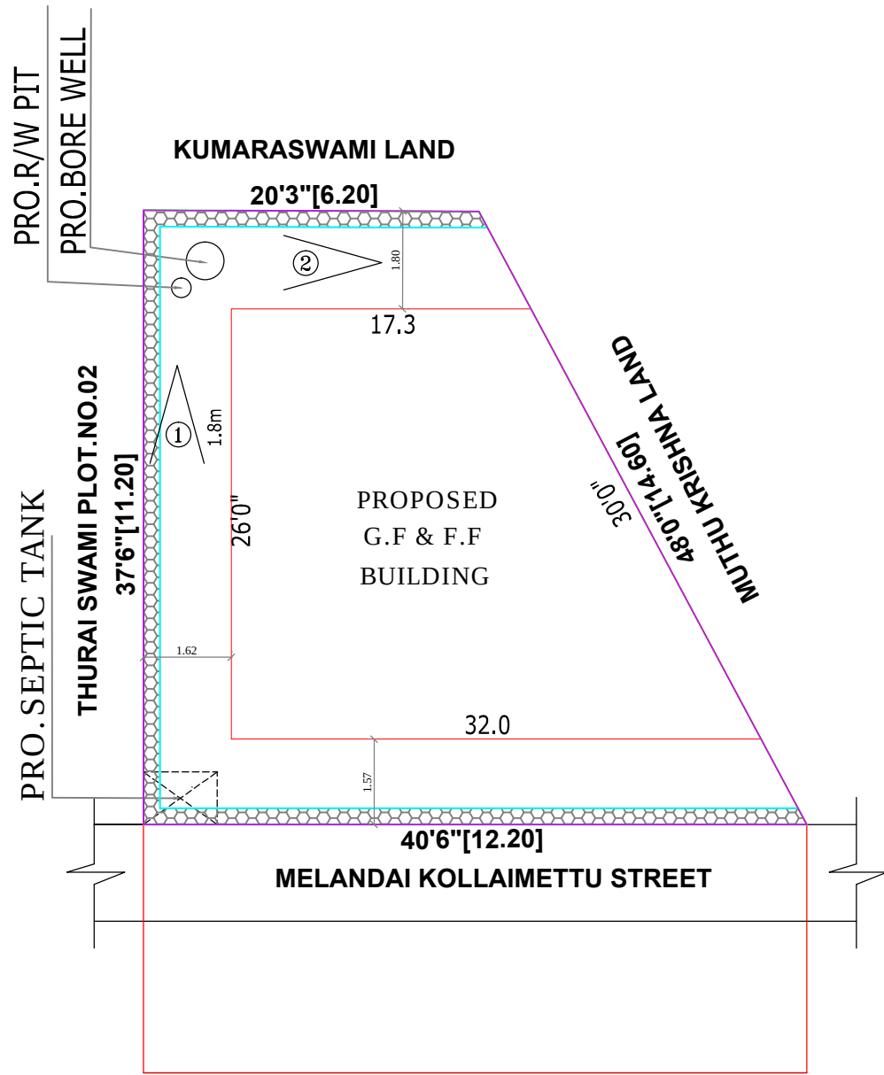
SITE PLAN
