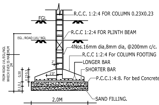
FOUNDATION DETAIL
