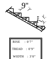
STAIRS DETAILS
