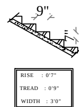
STAIRS DETAILS
