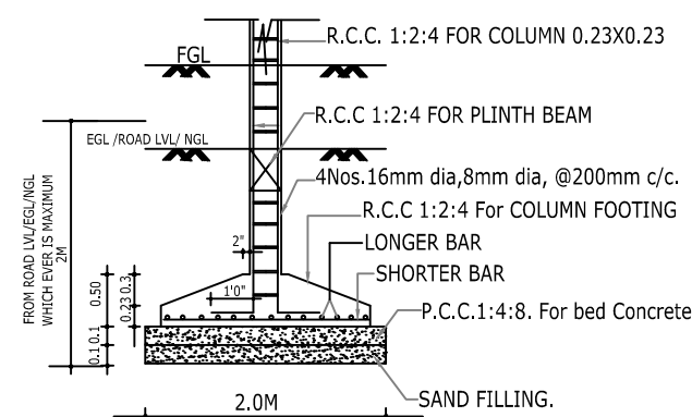
FOUNDATION DETAIL
