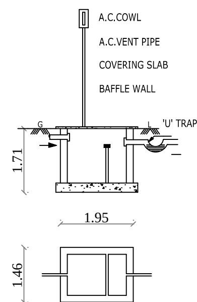
SEPTIC TANK
