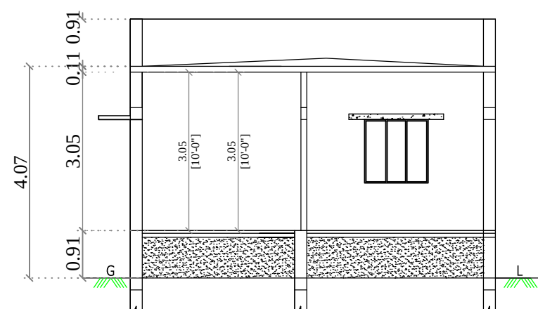
SECTION ON "SC"
