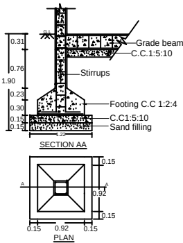
FOUNDATION DETAILS
