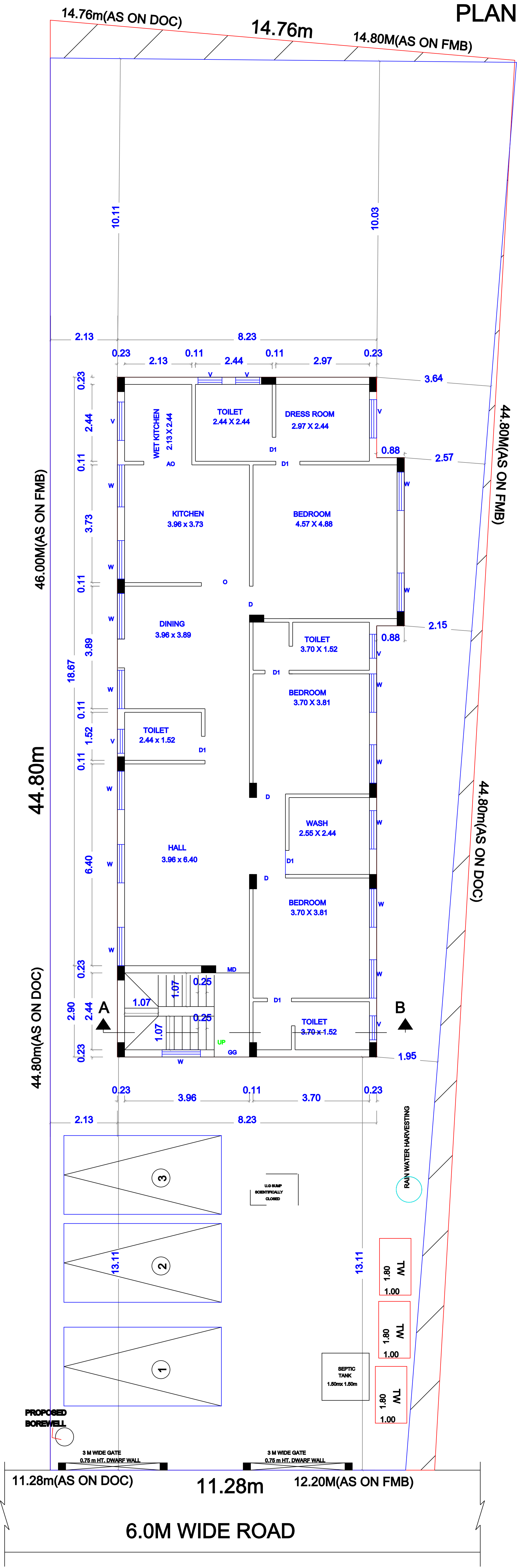
SITE/GROUND FLOOR PLAN (PROPOSED)
