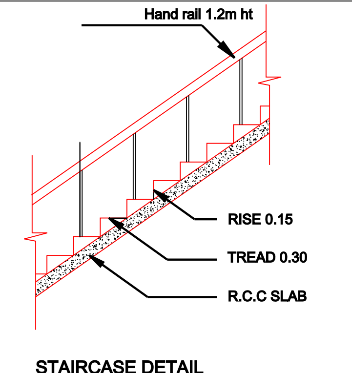
STAIRCASE DETAIL
