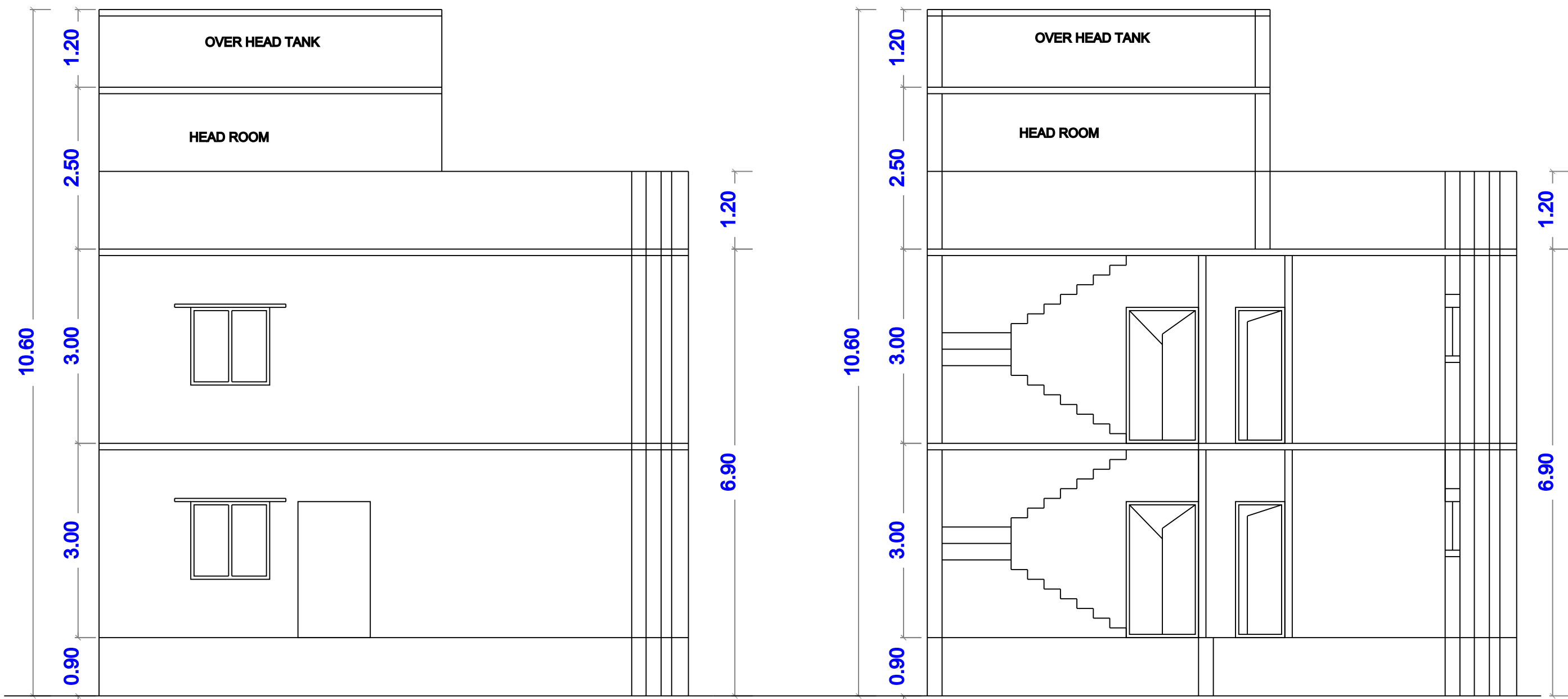
ELEVATION (PROPOSED)
