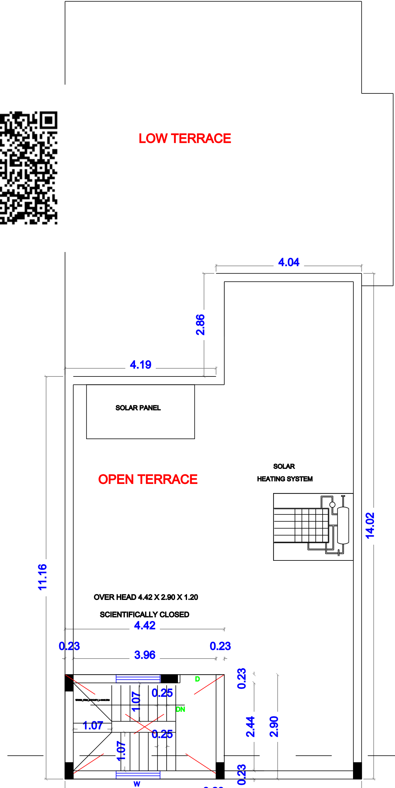
TERRACE FLOOR PLAN (PROPOSED)
