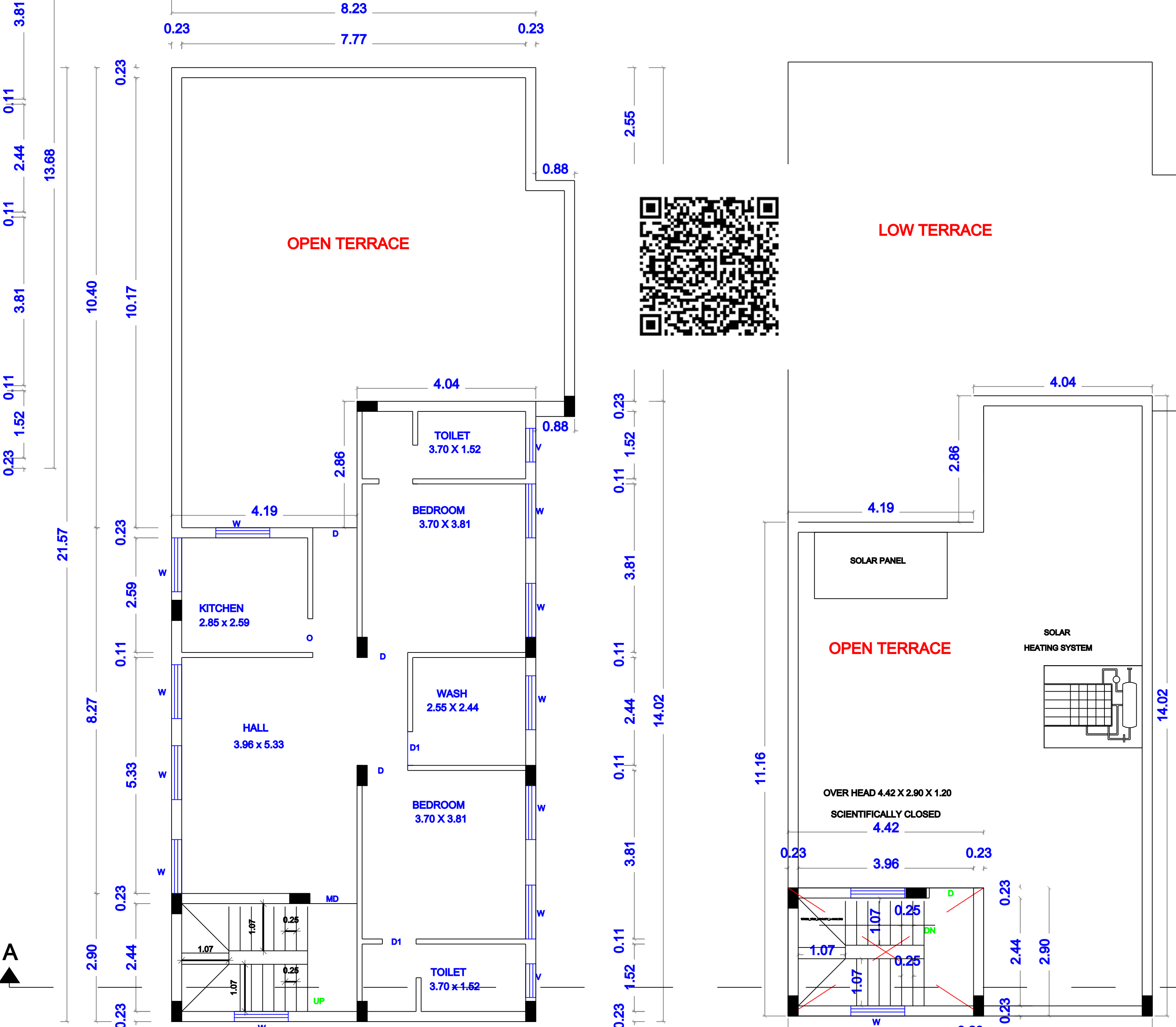
TERRACE FLOOR PLAN (PROPOSED)
