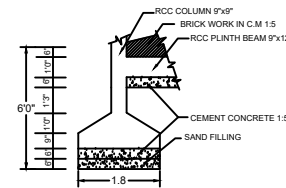
FOUNDATION DETAILS SCALE: 1/4 inches to a foot
