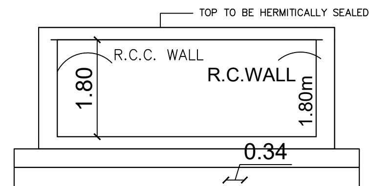
RWHS SECTION(SAMPLE) RWHS_CAPACITY_L=5000LTRS
