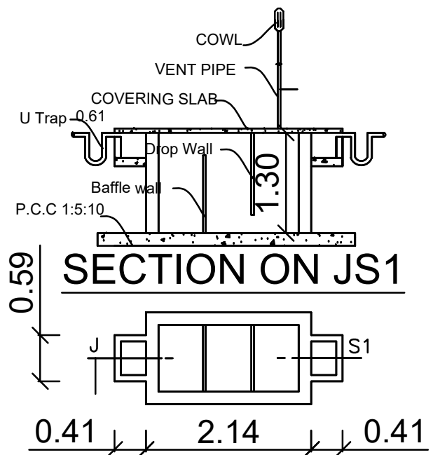
PLAN SEPTIC TANK DETAILS
