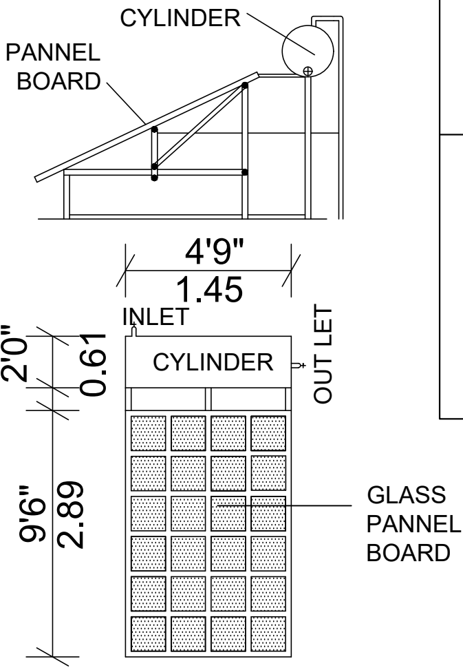
SOLAR WATER SYSTEM
