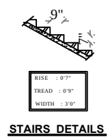
STAIRS DETAILS
