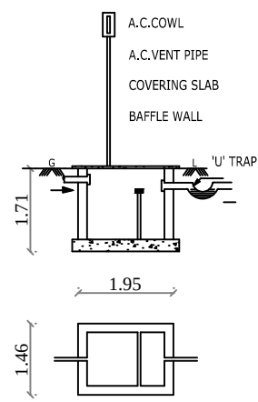
SEPTIC TANK
