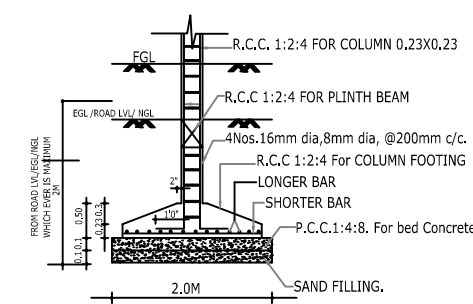
FOUNDATION DETAIL
