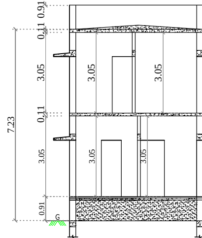
SECTION ON "SC"
