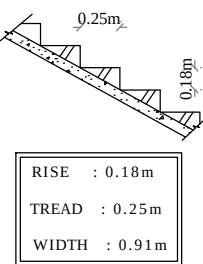
STAIRS DETAILS
