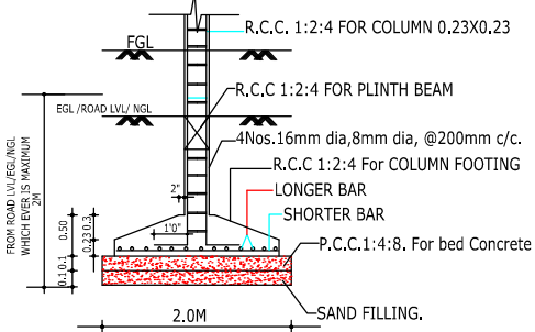
FOUNDATION DETAIL
