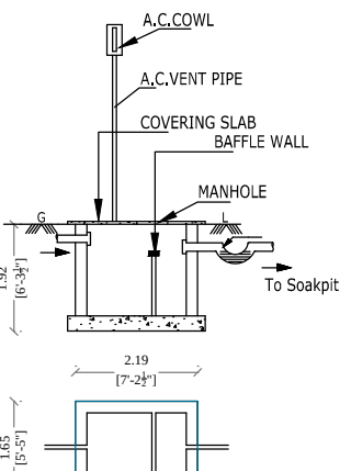
SEPTIC TANK
