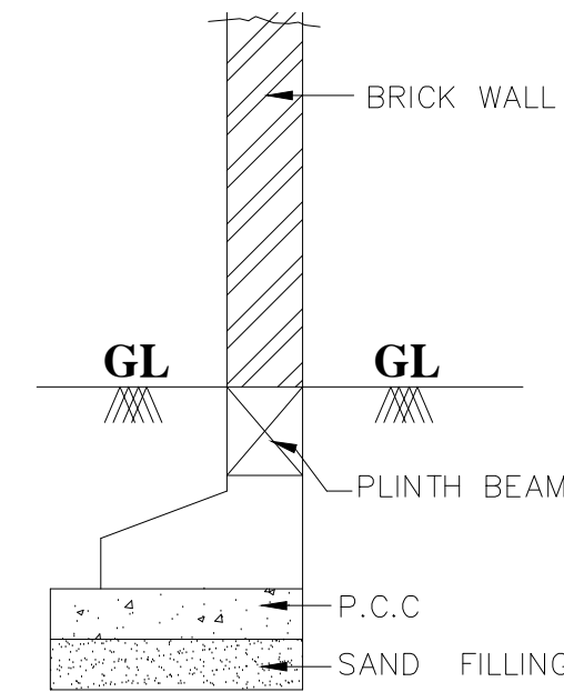
SECTION OF COMPOUND WALL
