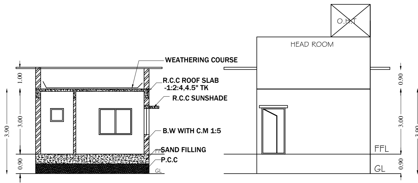
FRONT ELEVATION
