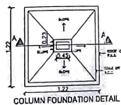
COLUMN FOUNDATION DETAIL
