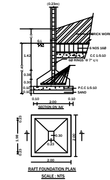
RAFT FOUNDATION PLAN
