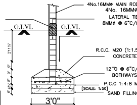
FOUNDATION DETAIL
