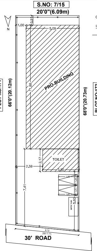
SITE PLAN
