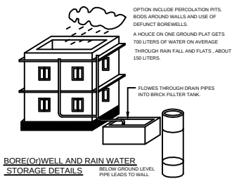
BOREWELL AND RAIN WATER STORAGE DETAILS
