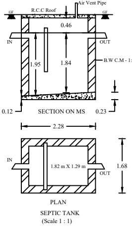
SECTION ON MS
