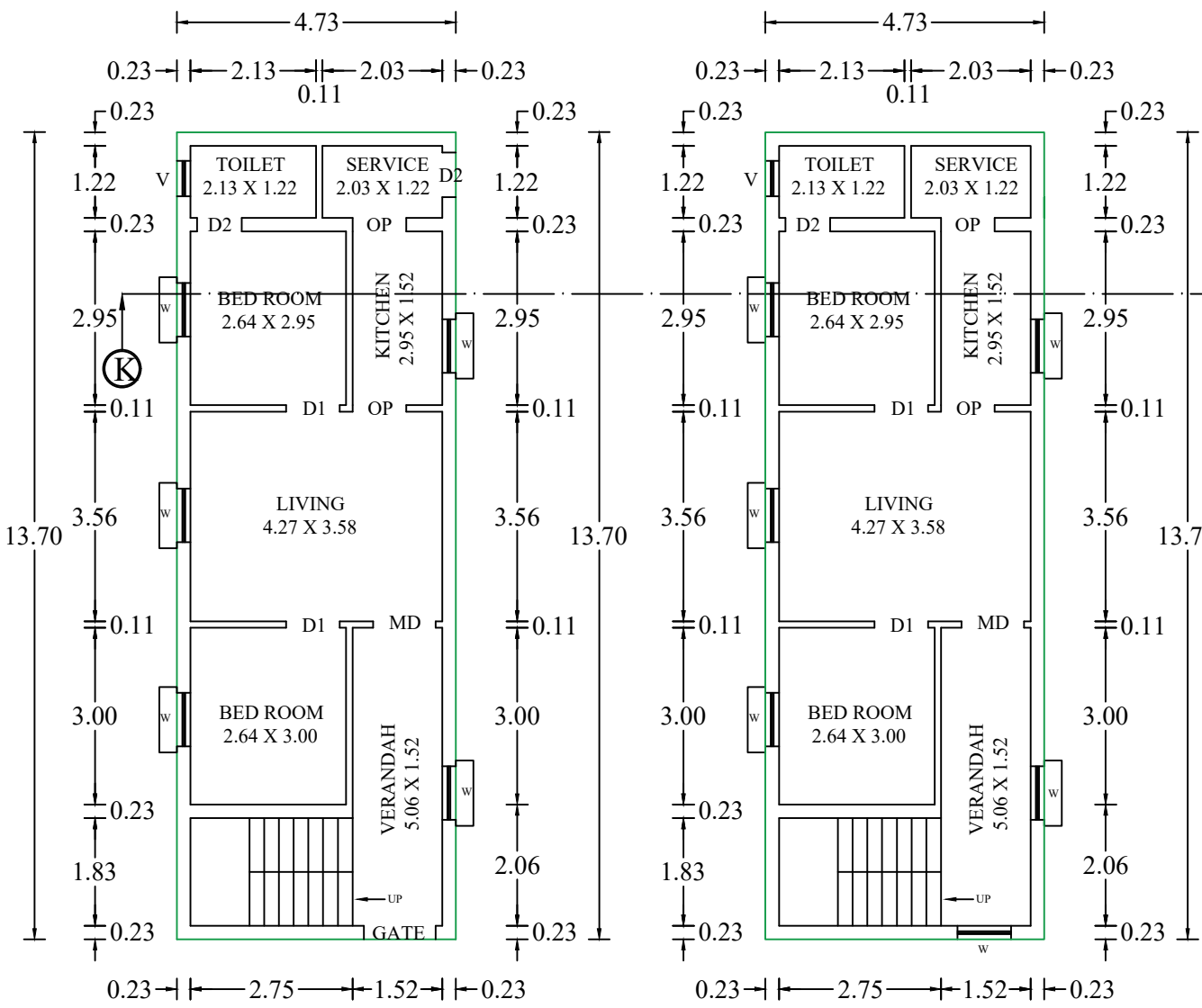
EXG. GROUND FLOOR PLAN
