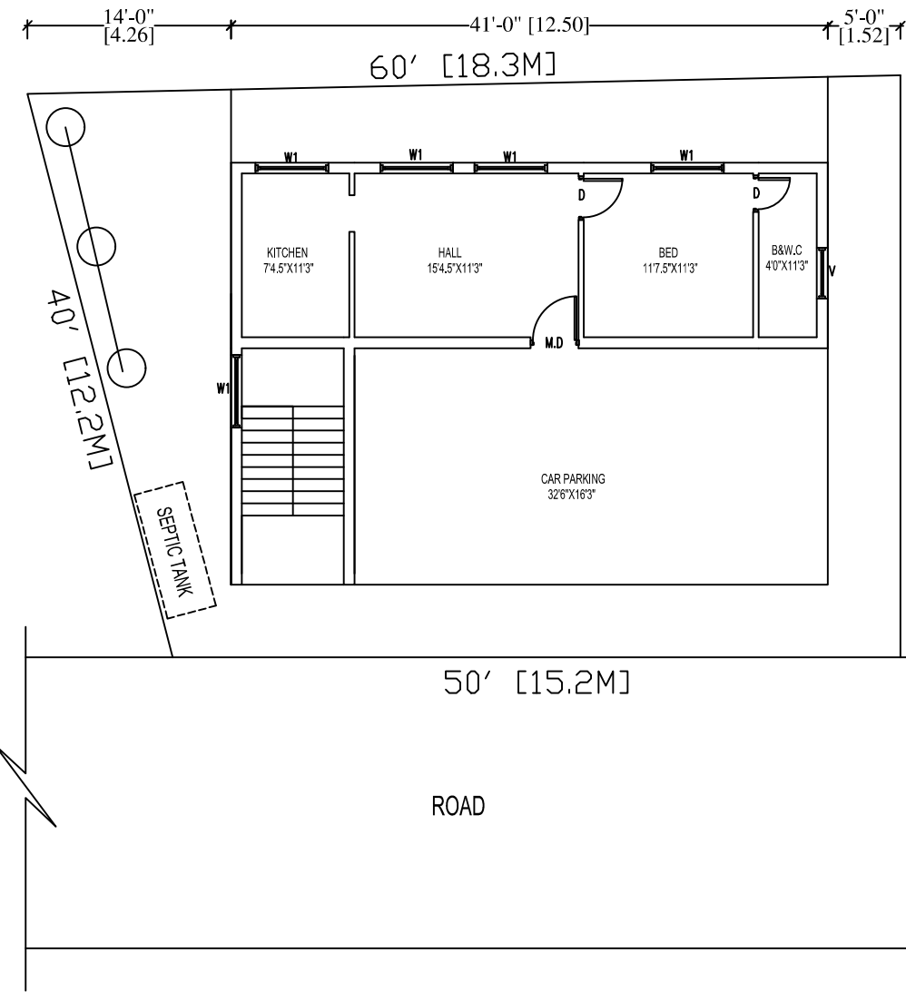
SITE CUM GROUND FLOOR PLAN
