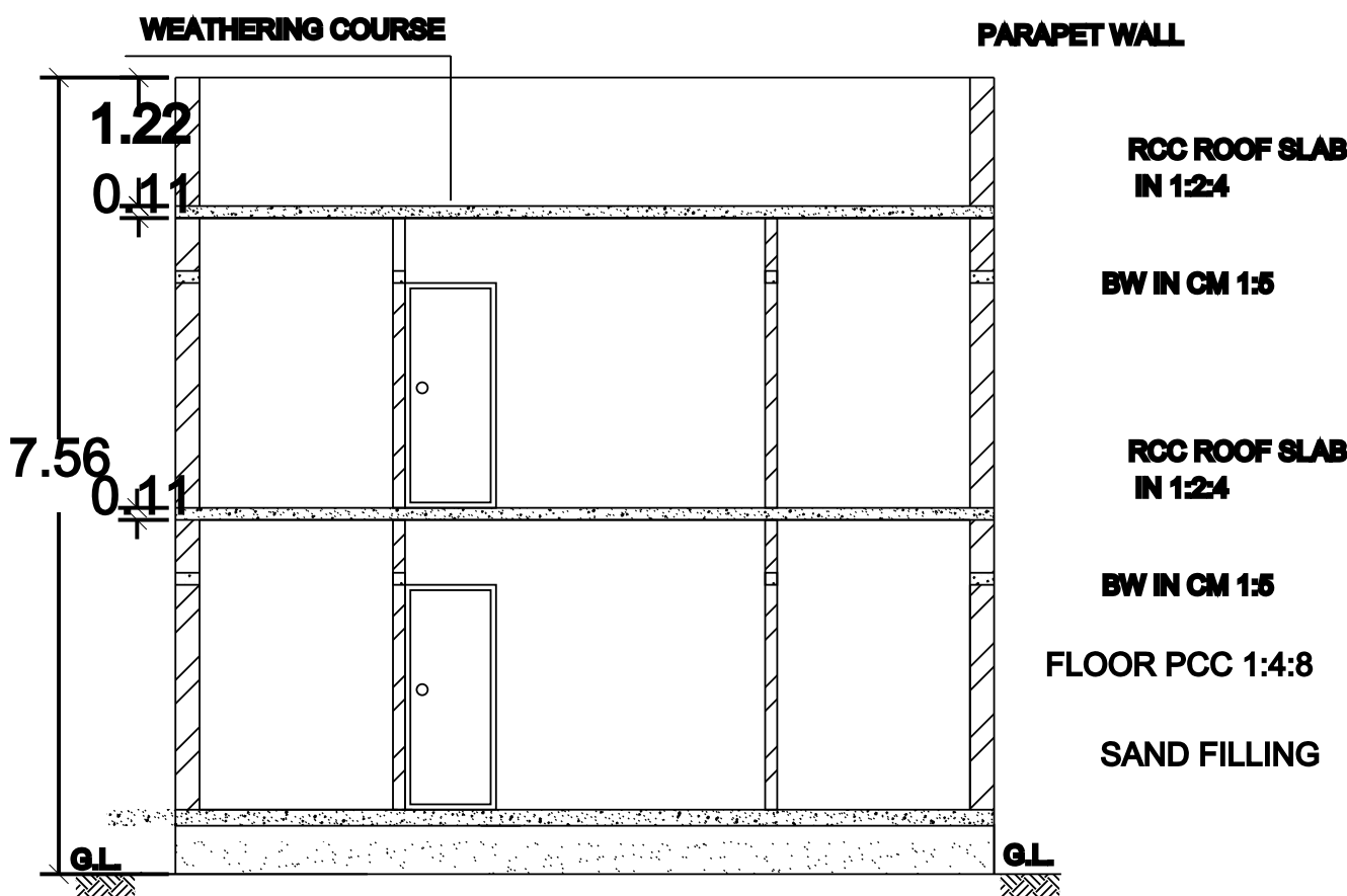
SECTIONAL VIEW E-V
