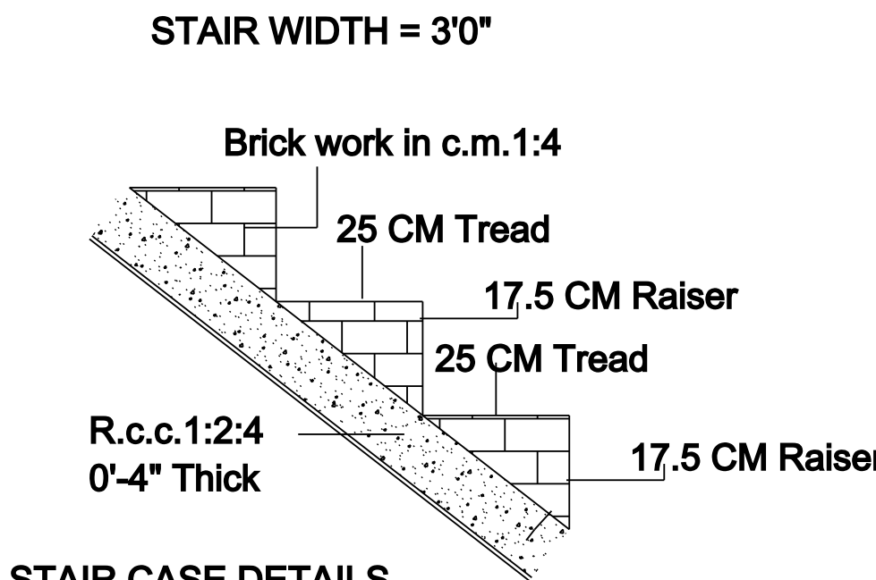
STAIR CASE DETAILS SCALE : 1" = 2'-0"
