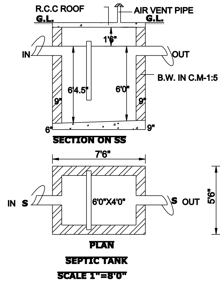
SEPTIC TANK SCALE 1"=8'0"
