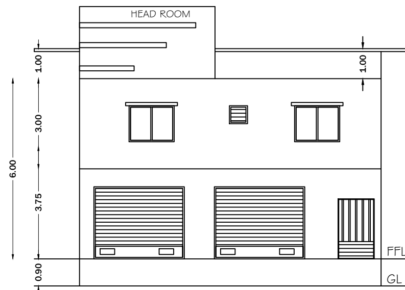
FRONT ELEVATION
