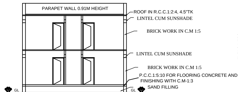
SECTION G-B
