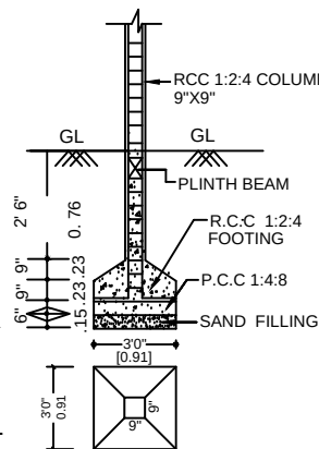
FOUNDATION DETAILS
