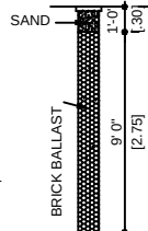
PERCOLATION PITS 12"Ø10"C/C
