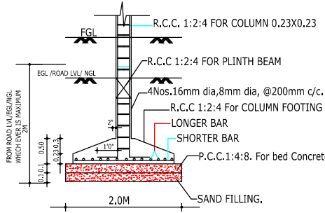
FOUNDATION DETAIL
