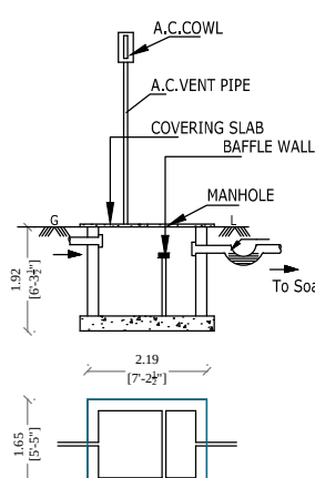
SEPTIC TANK
