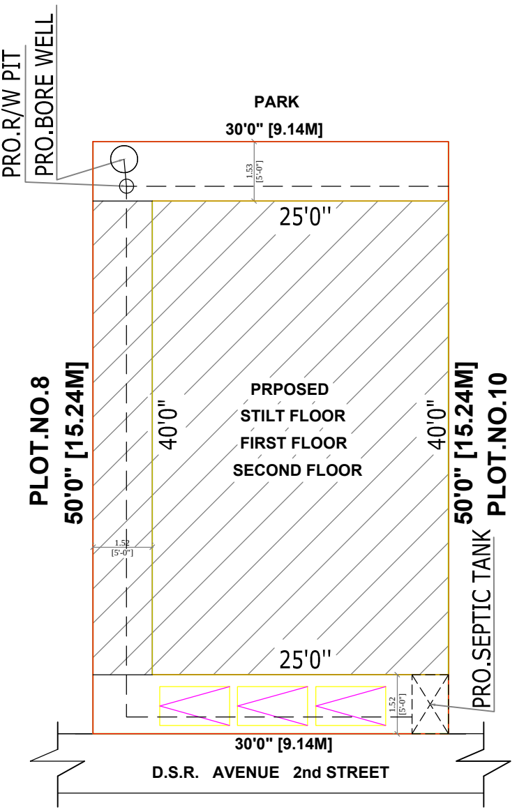
SITE PLAN SCALE: 1 INCH = 16 FEET
