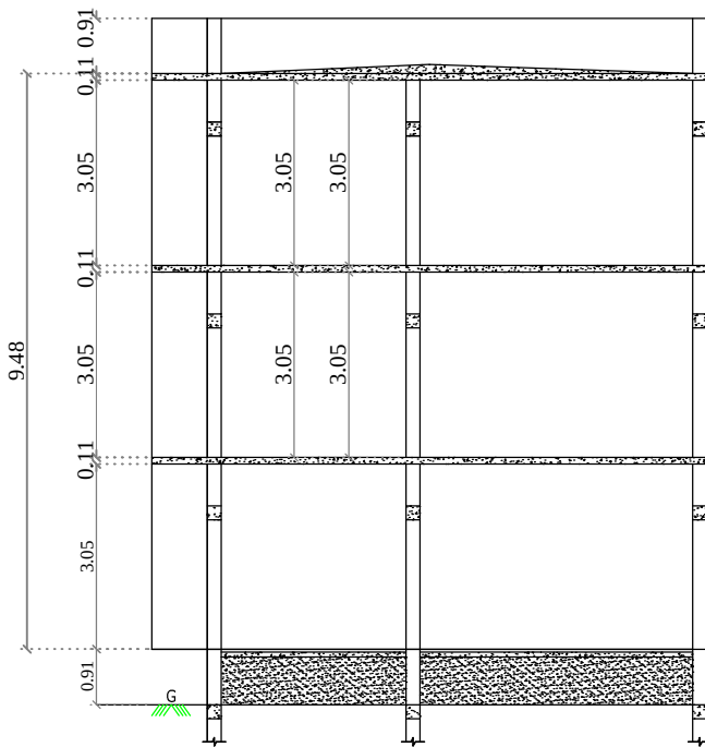
SECTION ON "SC"
