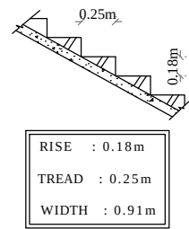
STAIRS DETAILS
