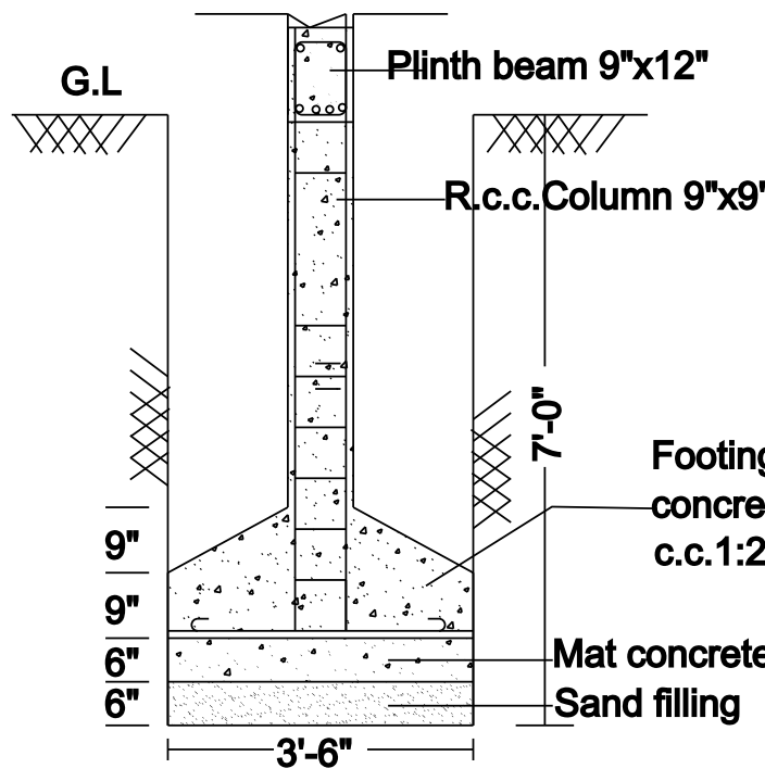
FOUNDATION DETAILS
