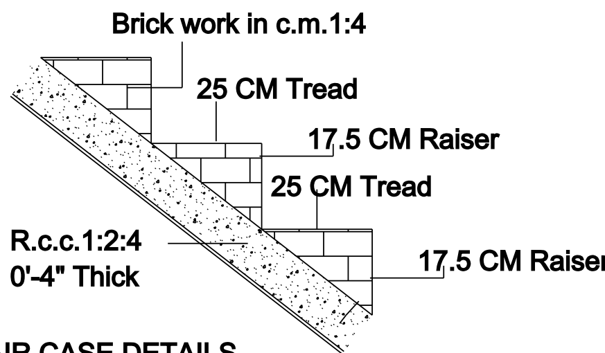
STAIR CASE DETAILS
