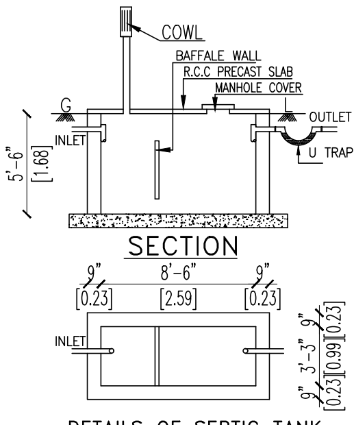
DETAILS OF SEPTIC TANK
