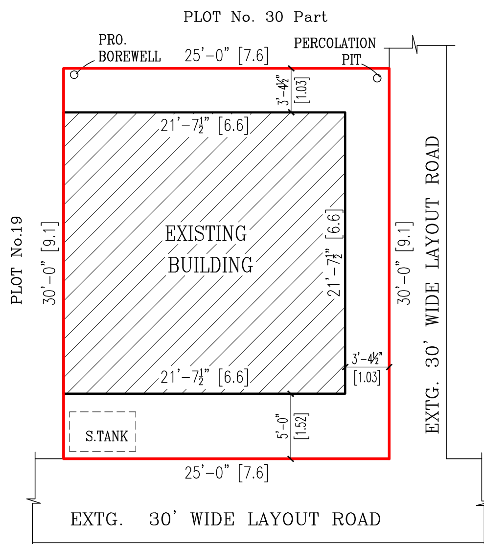
SITE PLAN
